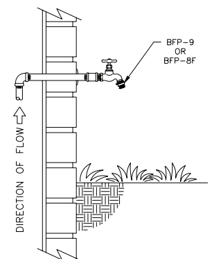
TYPICAL HOSE BIBB INSTALLATION
