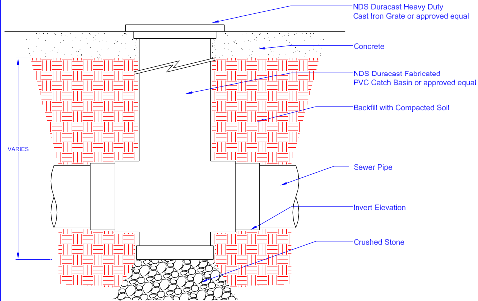
DURACAST ROUND GRATE WITH NDS DURACAST PVC CATCH BASIN CONNECTED TO A SEWER & DRAIN PIPE
